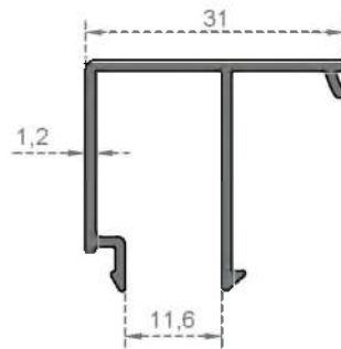
System Code 4021 Weight (kg/mt) 0,302
