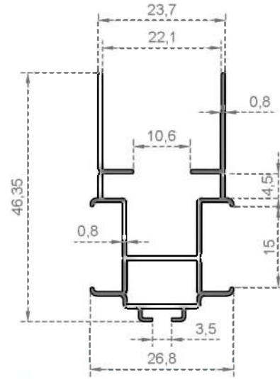
System Code 5020 Weight (kg/mt) 0,336
