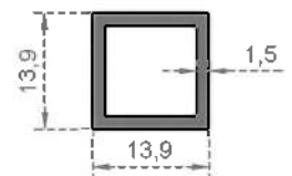
System Code 7036 Weight (kg/mt) 0,202
