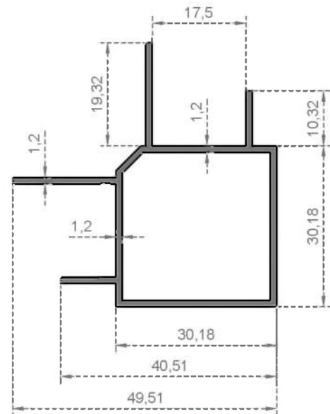
System Code 2910 Weight (kg/mt) 0,560
