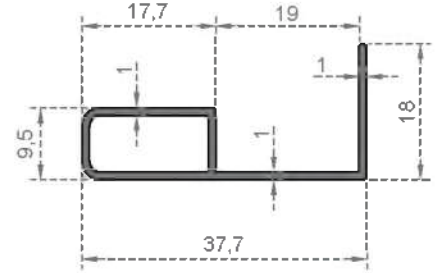
System Code 830 Weight (kg/mt) 0,232
