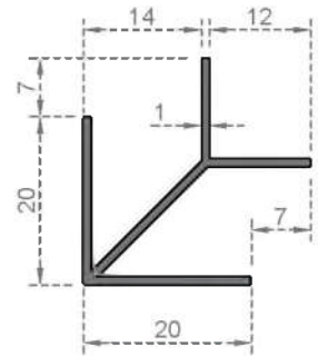
System Code 6561 Weight (kg/mt) 0,225
