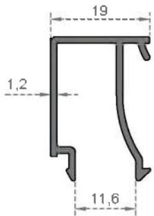
System Code 4027 Weight (kg/mt) 0,266
