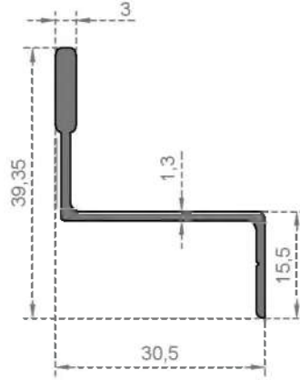
System Code 5009 Weight (kg/mt) 0,295
