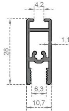
System Code 1576 Weight (kg/mt) 0,299
