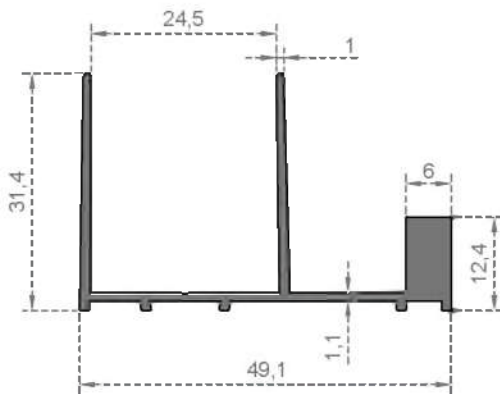
System Code 2987 Weight (kg/mt) 0,520
