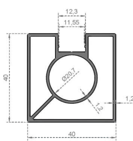
System Code 7033 Weight (kg/mt) 0,825
