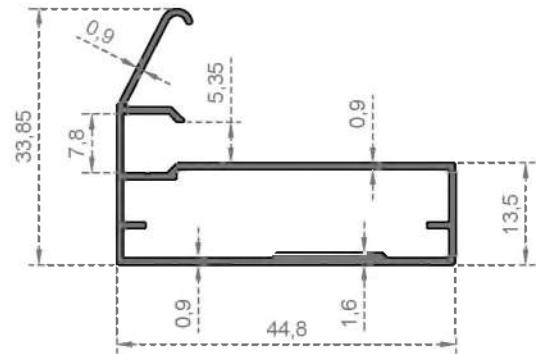
System Code 832 Weight (kg/mt) 0,401
