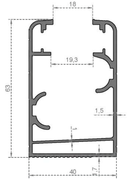
System Code 239 Weight (kg/mt) 1,128
