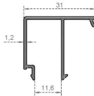
System Code 4021 Weight (kg/mt) 0,302
