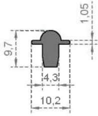
System Code 5697 Weight (kg/mt) 0,126
