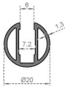
System Code 1571 Weight (kg/mt) 0,299
