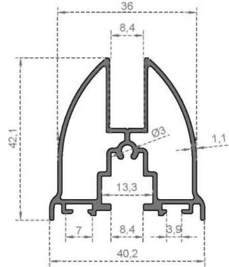
System Code 240 Weight (kg/mt) 0,702
