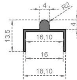
System Code 6944 Weight (kg/mt) 0,135
