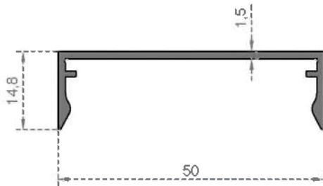
System Code 509 Weight (kg/mt) 0,325
