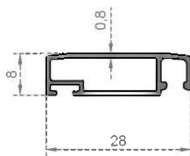
System Code 826 Weight (kg/mt) 0,165
