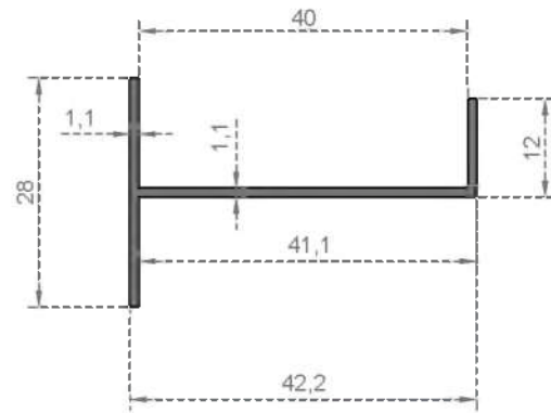
System Code 7044 Weight (kg/mt) 0,240
