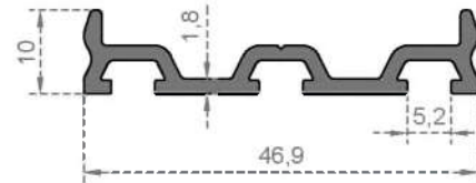
System Code 510 Weight (kg/mt) 0,395
