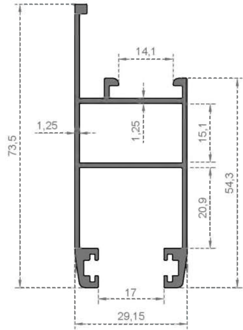
System Code 3001 Weight (kg/mt) 0,795
