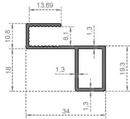
System Code 235 Weight (kg/mt) 0,360
