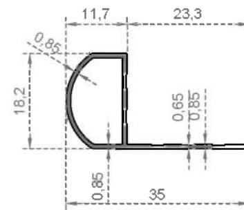
System Code 827 Weight (kg/mt) 0,165
