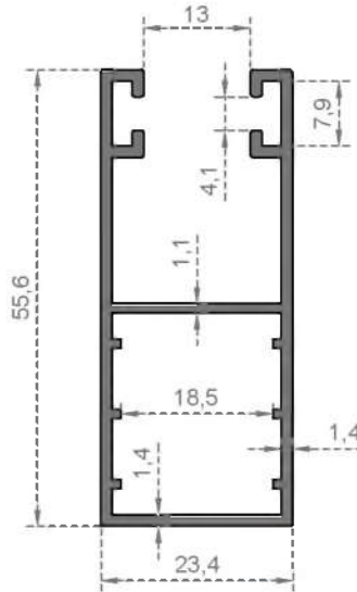
System Code 5018 Weight (kg/mt) 0,666
