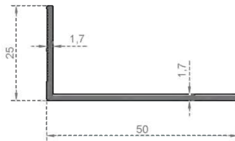
System Code 6554 Weight (kg/mt) 0,331
