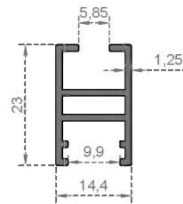
System Code 2986 Weight (kg/mt) 0,275
