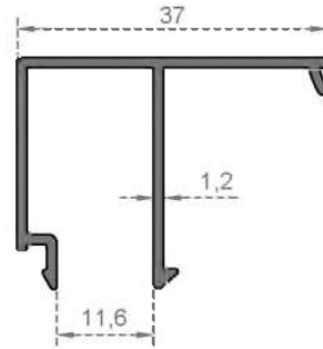
System Code 4018 Weight (kg/mt) 0,321
