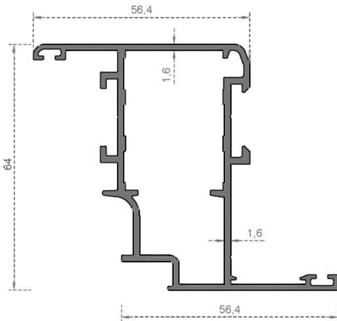
System Code 8002 Weight (kg/mt) 1,258
