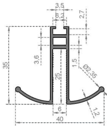
System Code 2998 Weight (kg/mt) 0,385
