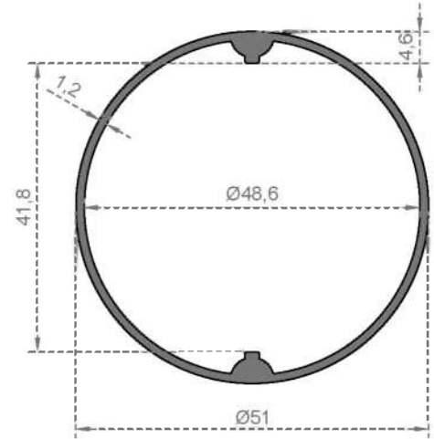
System Code 819 Weight (kg/mt) 0,582
