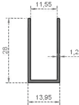
System Code 1392 Weight (kg/mt) 0,219
