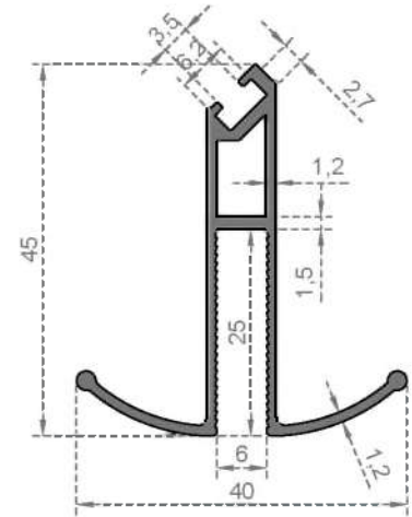
System Code 2999 Weight (kg/mt) 0,455
