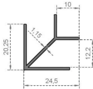
System Code 6559 Weight (kg/mt) 0,245
