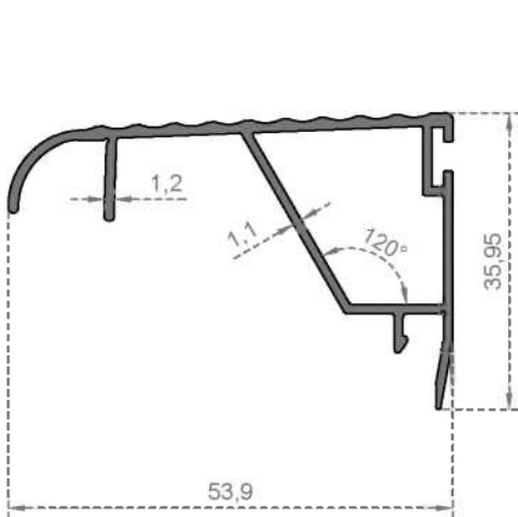
System Code 6945 Weight (kg/mt) 0,480
