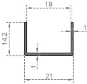
System Code 828 Weight (kg/mt) 0,128
