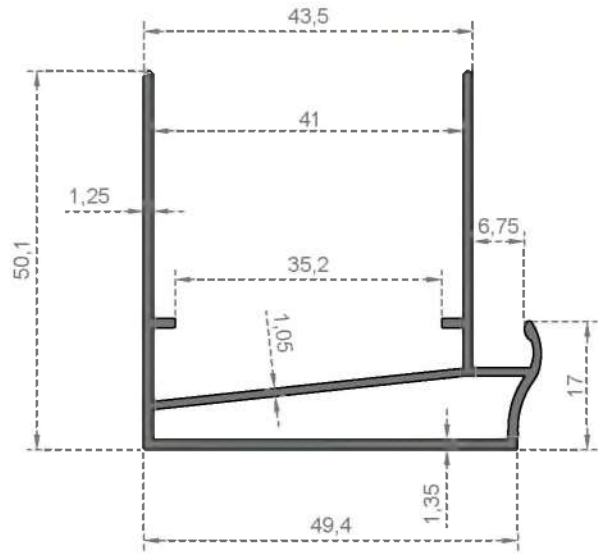
System Code 257 Weight (kg/mt) 0,700
