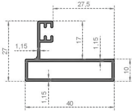
System Code 204 Weight (kg/mt) 0,410
