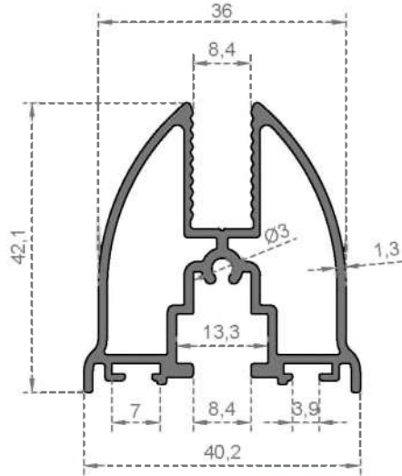
System Code 202 Weight (kg/mt) 0,812
