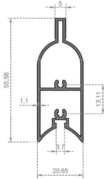
System Code 2962 Weight (kg/mt) 0,572
