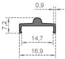
System Code 5945 Weight (kg/mt) 0,092
