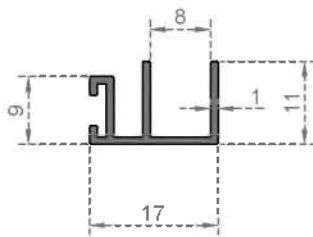
System Code 206 Weight (kg/mt) 0,136
