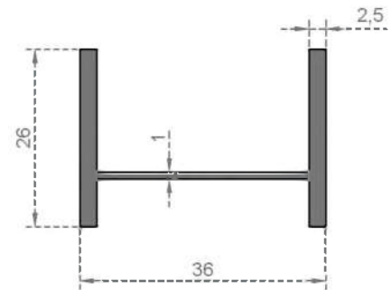
System Code 6709 Weight (kg/mt) 0,437
