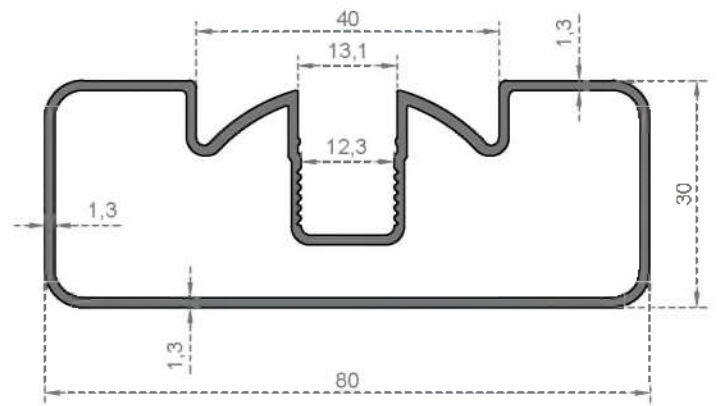
System Code 7038 Weight (kg/mt) 0,936
