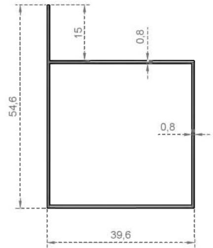
System Code 801 Weight (kg/mt) 0,369
