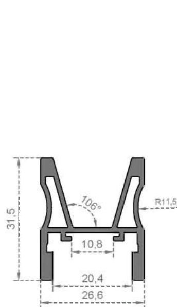
System Code 6734 Weight (kg/mt) 0,560
