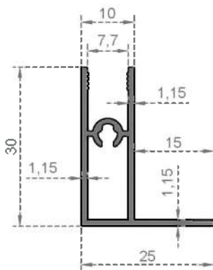
System Code 2961 Weight (kg/mt) 0,303
