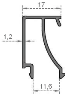
System Code 4028 Weight (kg/mt) 0,263
