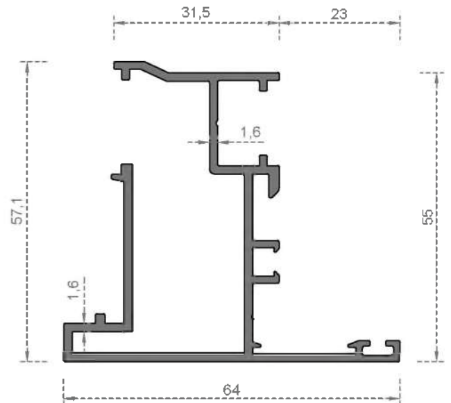
System Code 8009 Weight (kg/mt) 1,015
