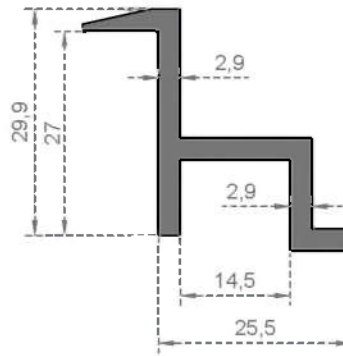
System Code 6723 Weight (kg/mt) 0,565
