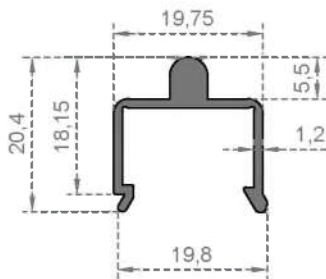
System Code 420 Weight (kg/mt) 0,230
