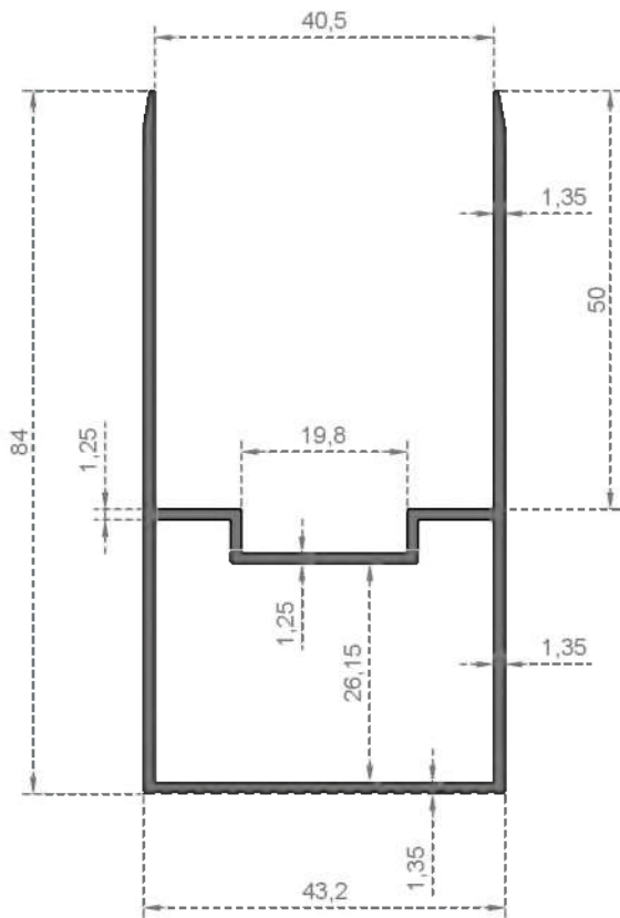
System Code 215 Weight (kg/mt) 0,910
