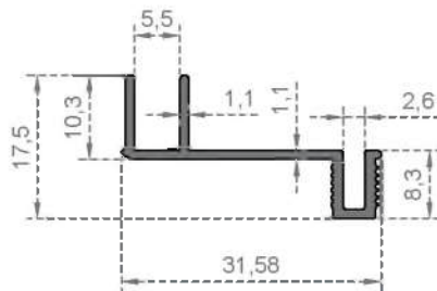
System Code 2916 Weight (kg/mt) 0,201
