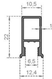
System Code 1831 Weight (kg/mt) 0,189
