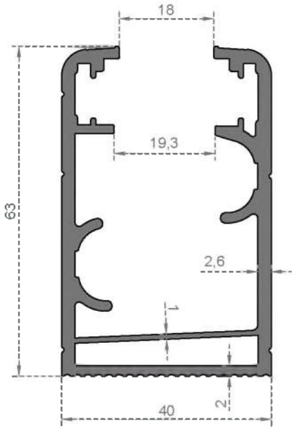
System Code 200 Weight (kg/mt) 1,495
