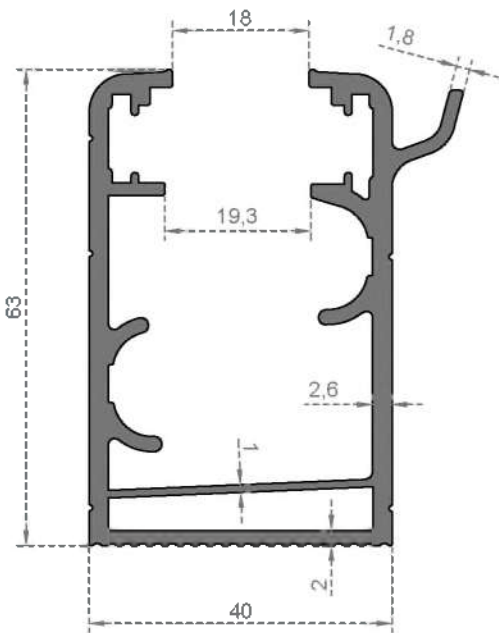
System Code 201 Weight (kg/mt) 1,565
