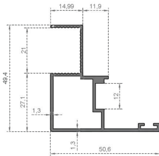
System Code 242 Weight (kg/mt) 0,618
