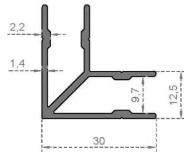
System Code 421 Weight (kg/mt) 0,465
