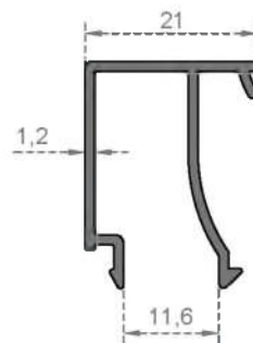
System Code 4026 Weight (kg/mt) 0,275
