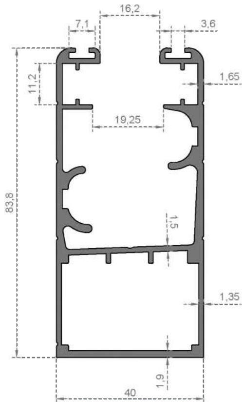
System Code 228 Weight (kg/mt) 1,556
