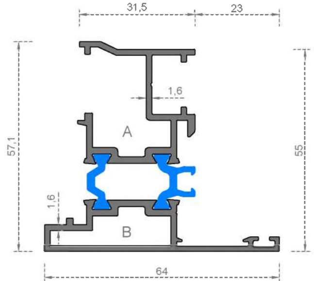
System Code 4009 Weight (kg/mt) 1.325
