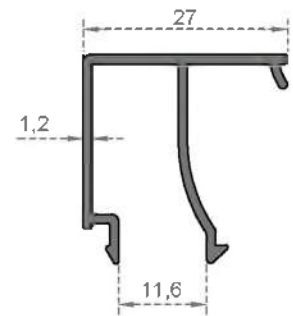
System Code 4023 Weight (kg/mt) 0,292
