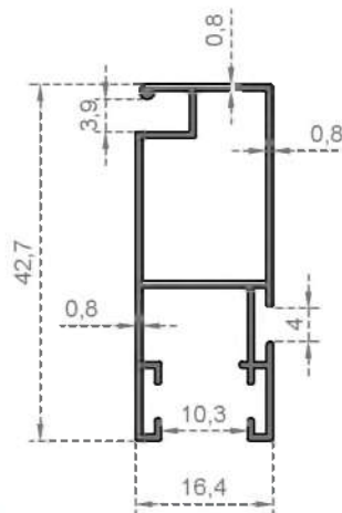
System Code 5564 Weight (kg/mt) 0,314
