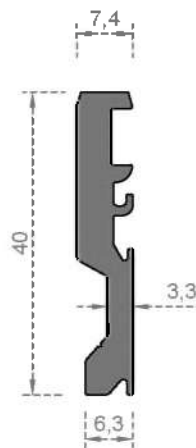
System Code 4015 Weight (kg/mt) 0,542
