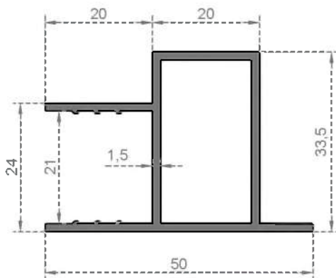
System Code 6687 Weight (kg/mt) 0,625
