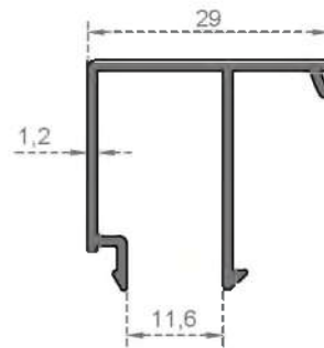
System Code 4022 Weight (kg/mt) 0,295
