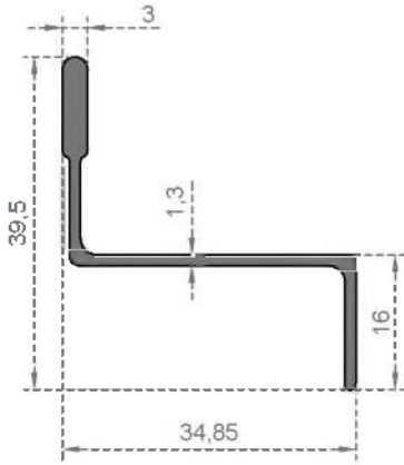
System Code 5007 Weight (kg/mt) 0,310
