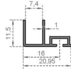
System Code 3105 Weight (kg/mt) 0,145
