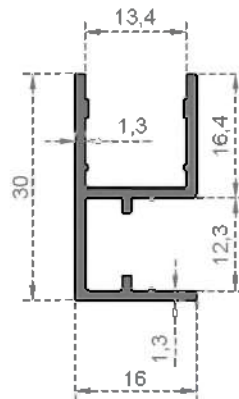
System Code 7051 Weight (kg/mt) 0,290
