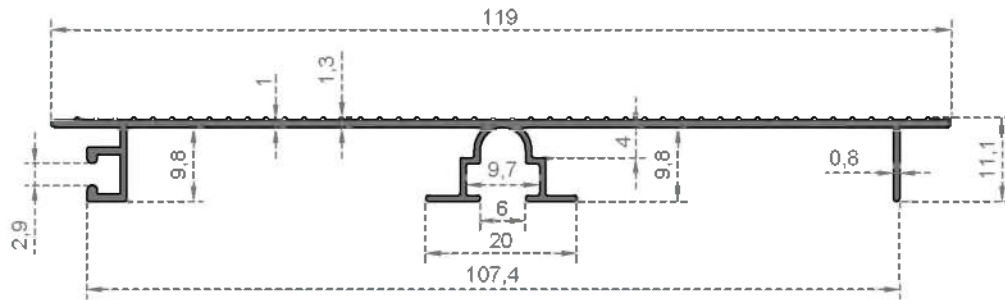
System Code 810 Weight (kg/mt) 0,494
