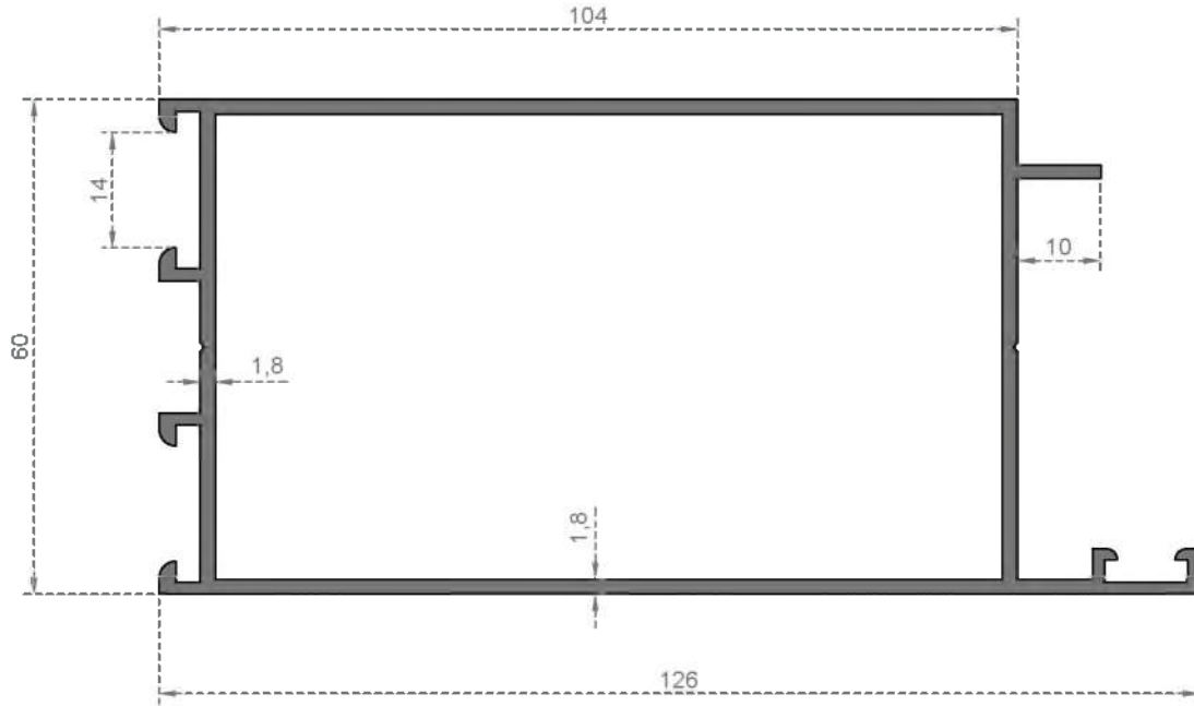
WIDE CASEMENT
