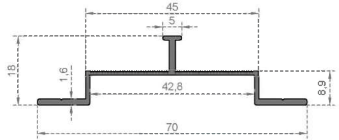
System Code 6551 Weight (kg/mt) 0,320
