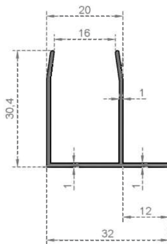
System Code 2575 Weight (kg/mt) 0,246
