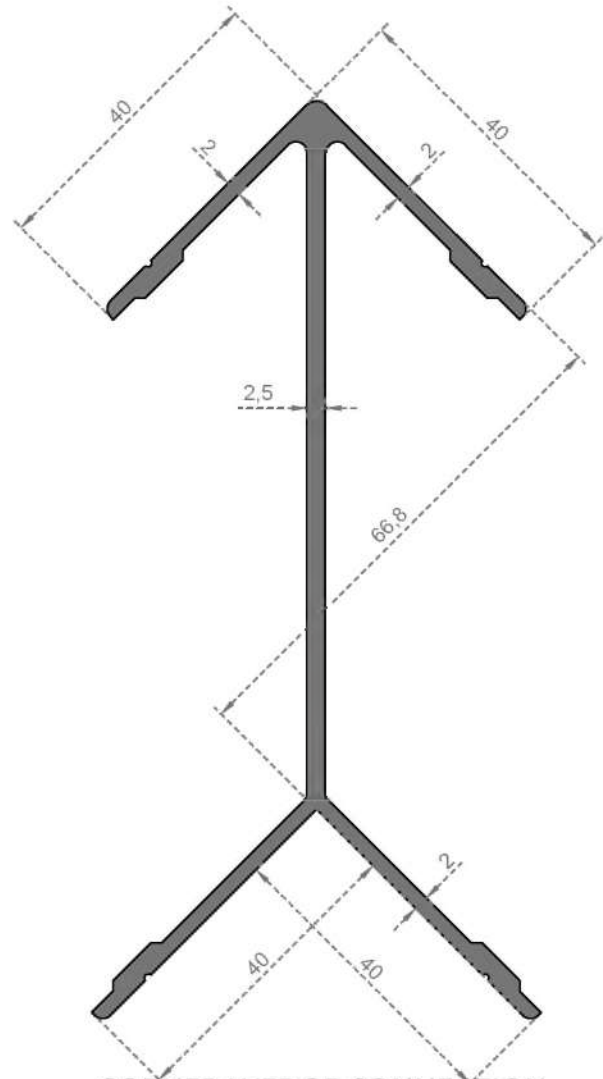
CORNER WEDGE CONNECTION
