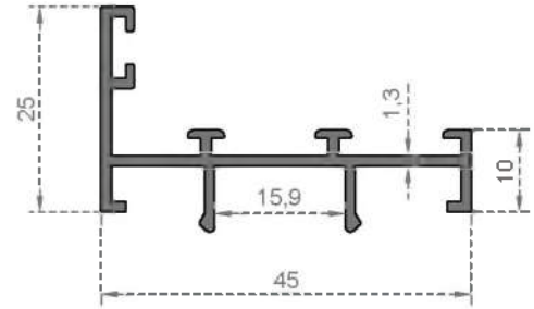
System Code 416 Weight (kg/mt) 0,412
