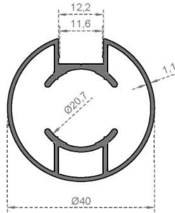
System Code 7003 Weight (kg/mt) 0,631
