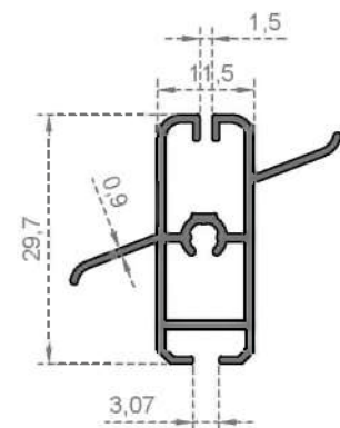
System Code 2993 Weight (kg/mt) 0,327
