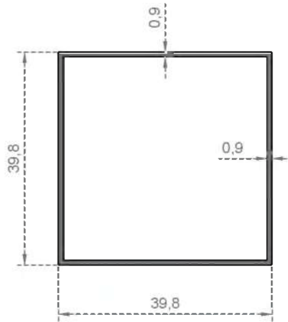
System Code 6936 Weight (kg/mt) 0,380
