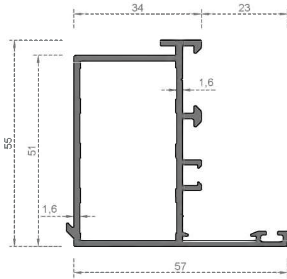
System Code 8006 Weight (kg/mt) 0,980
