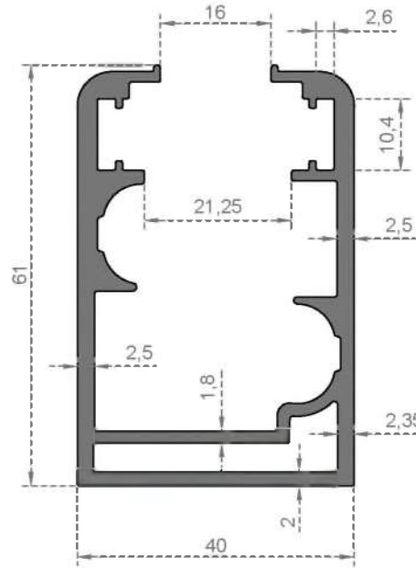
System Code 7106 Weight (kg/mt) 1,535
