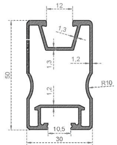
System Code 6729 Weight (kg/mt) 0,795
