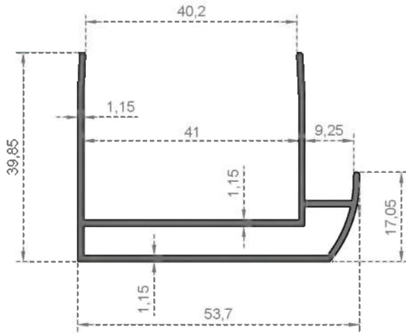
System Code 214 Weight (kg/mt) 0,583
