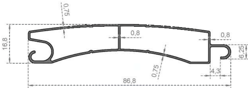
System Code 5025 Weight (kg/mt) 0,475
