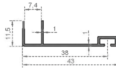
System Code 3106 Weight (kg/mt) 0,205
