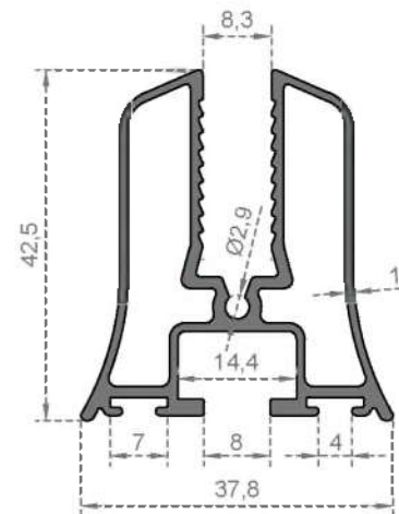
System Code 245 Weight (kg/mt) 0,745
