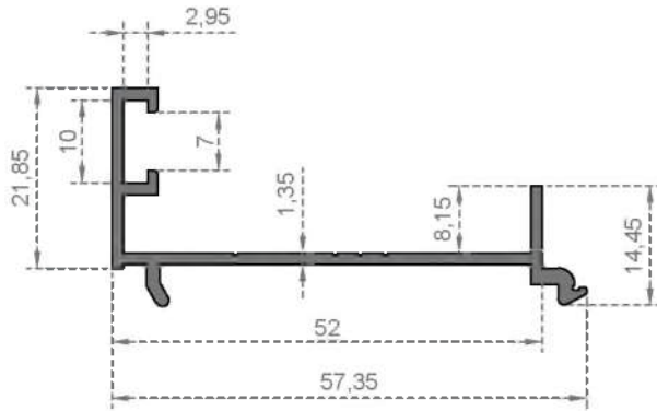
CASEMENT ADAPTER
