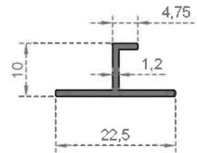
System Code 6555 Weight (kg/mt) 0,115
