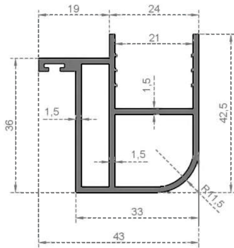
System Code 6684 Weight (kg/mt) 0,785
