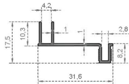
System Code 2946 Weight (kg/mt) 0,180
