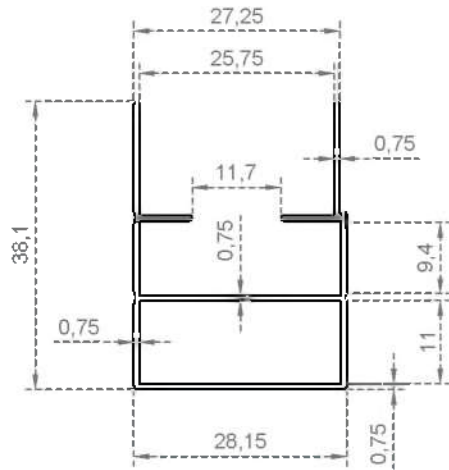
System Code 5019 Weight (kg/mt) 0,292
