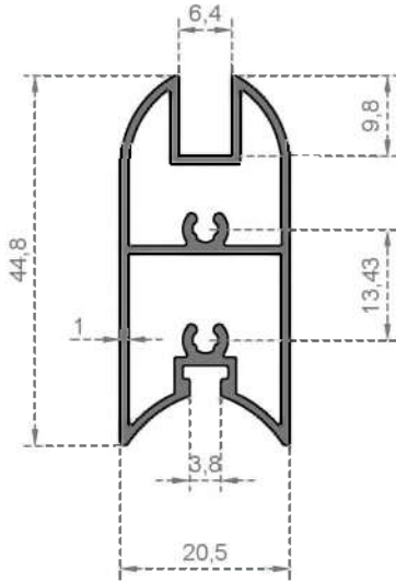
System Code 2222 Weight (kg/mt) 0,530
