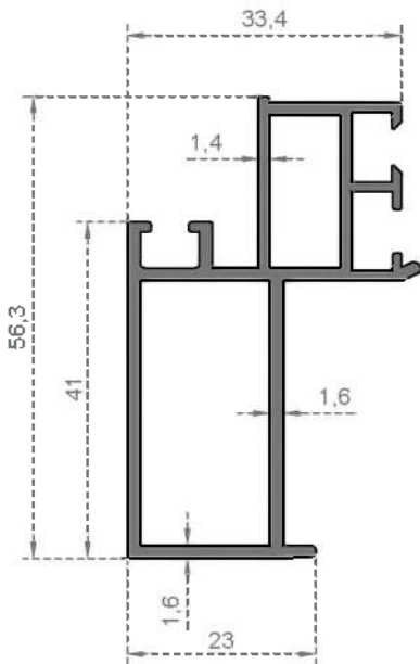
System Code 504 Weight (kg/mt) 0,835
