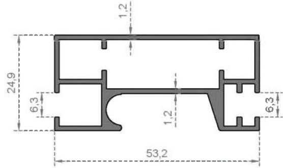
System Code 2984 Weight (kg/mt) 0,715
