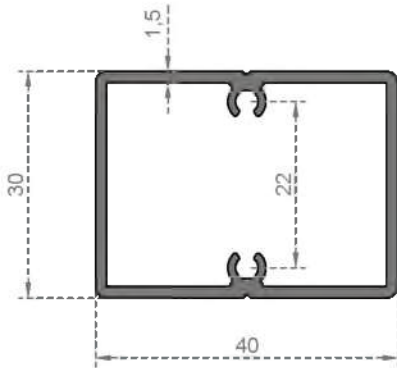
System Code 6708 Weight (kg/mt) 0,600
