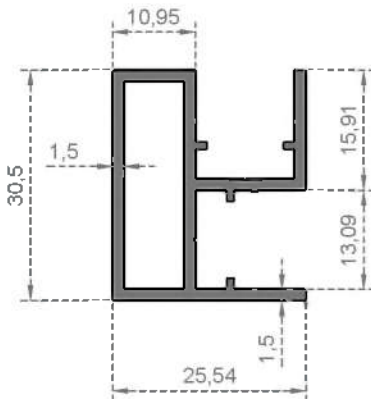
System Code 7040 Weight (kg/mt) 0,510
