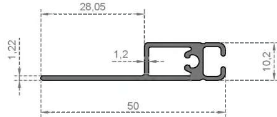
System Code 1720 Weight (kg/mt) 0,334
