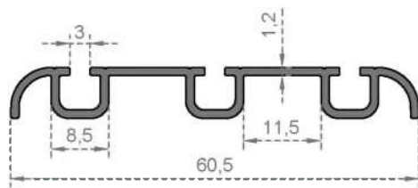
System Code 256 Weight (kg/mt) 0,365
