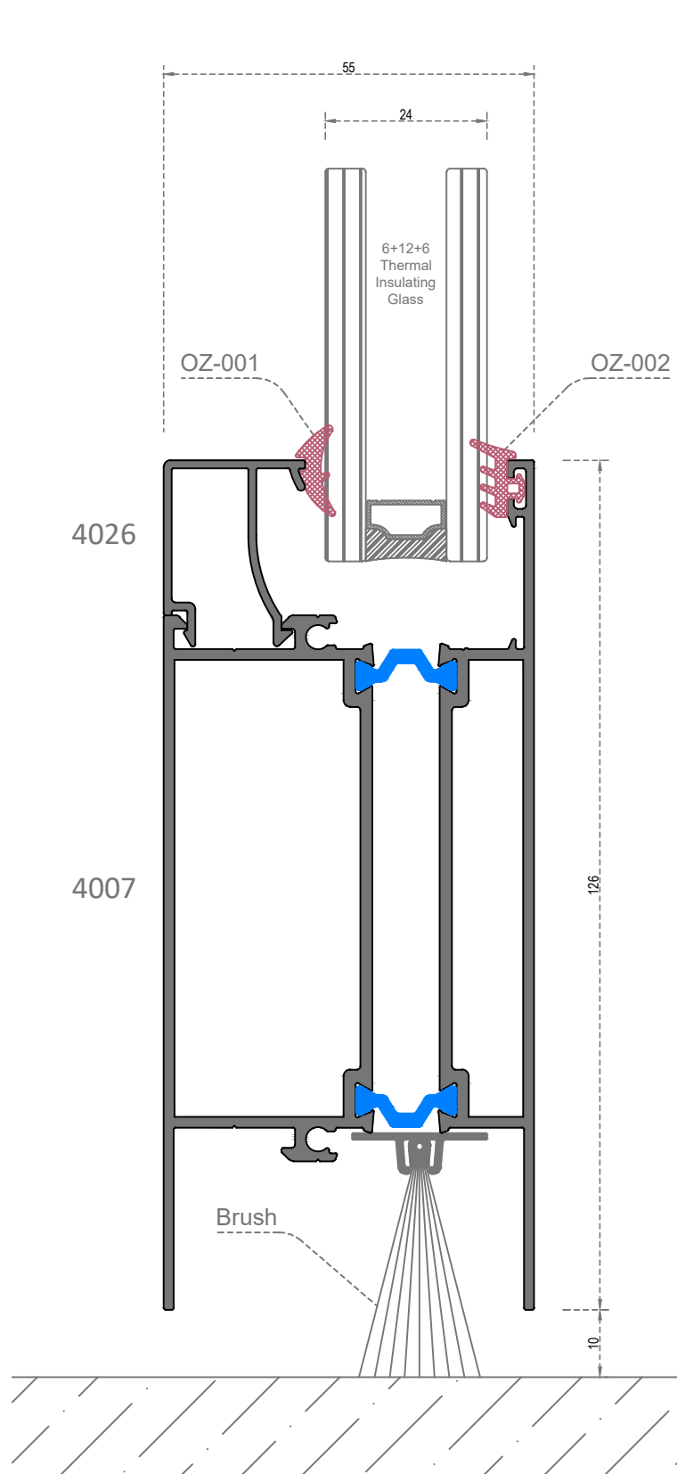
DETAIL-1
