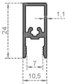
System Code 1516 Weight (kg/mt) 0,241
