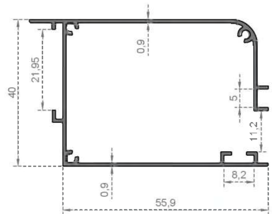
System Code 6533 Weight (kg/mt) 0,530
