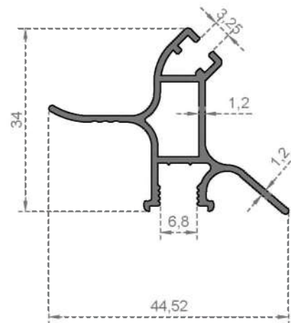
System Code 1945 Weight (kg/mt) 0,419
