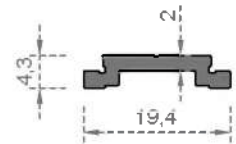
System Code 614 Weight (kg/mt) 0,130
