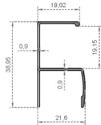
System Code 1955 Weight (kg/mt) 0,242
