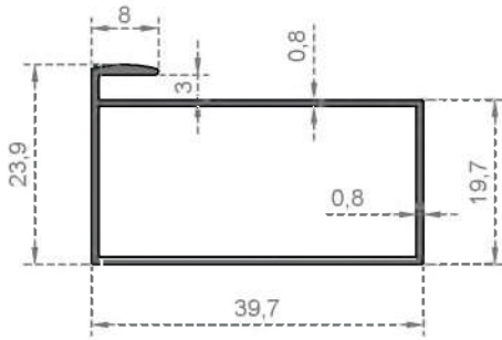
System Code 802 Weight (kg/mt) 0,280
