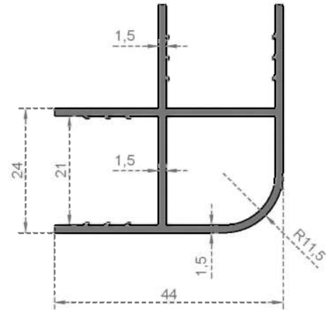
System Code 6685 Weight (kg/mt) 0,690
