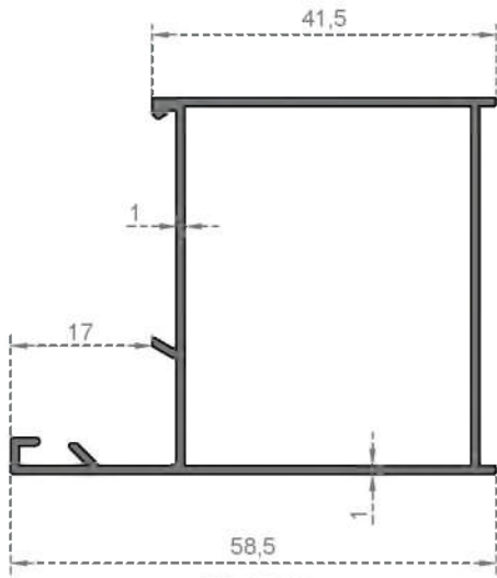
FRAME
