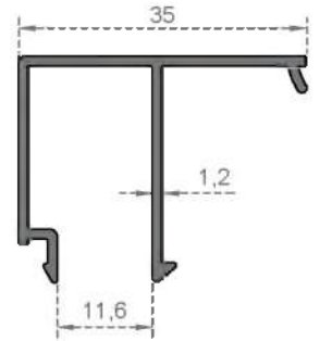
System Code 4019 Weight (kg/mt) 0,315
