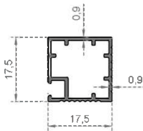
System Code 811 Weight (kg/mt) 0,188
