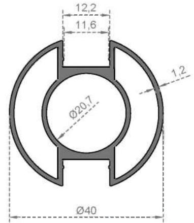
System Code 7011 Weight (kg/mt) 0,720
