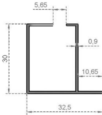
System Code 2989 Weight (kg/mt) 0,256
