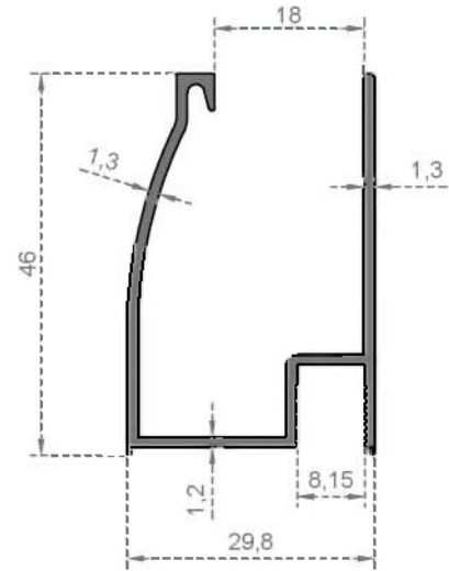
System Code 2906 Weight (kg/mt) 0,458
