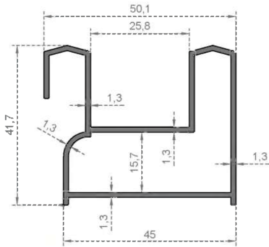
System Code 3000 Weight (kg/mt) 0,724
