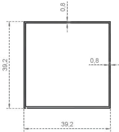
System Code 800 Weight (kg/mt) 0,333
