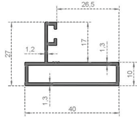
System Code 225 Weight (kg/mt) 0,430
