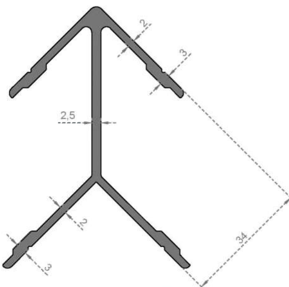
CORNER WEDGE CONNECTION
