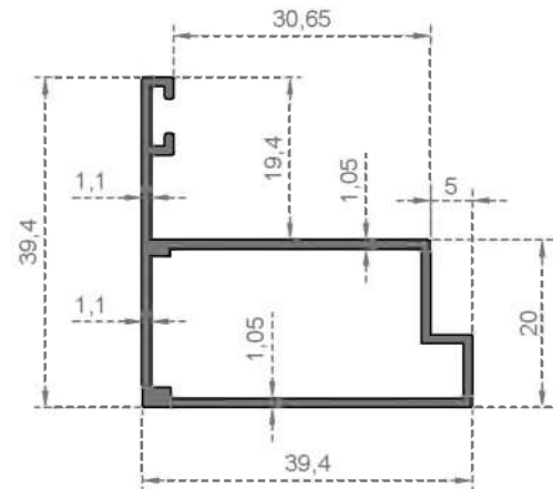
System Code 227 Weight (kg/mt) 0,430
