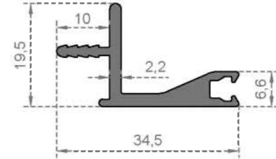
System Code 809 Weight (kg/mt) 0,375
