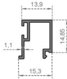
System Code 418 Weight (kg/mt) 0,180
