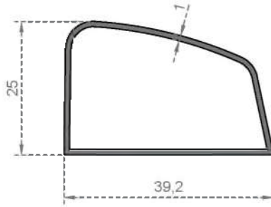
System Code 2047 Weight (kg/mt) 0,304
