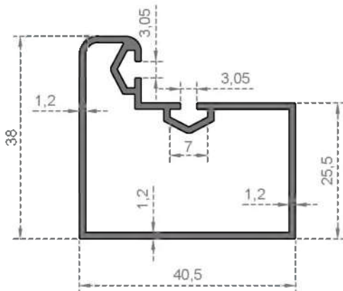
System Code 219 Weight (kg/mt) 0,552
