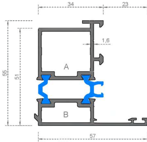
System Code 4006 Weight (kg/mt) 1.335
