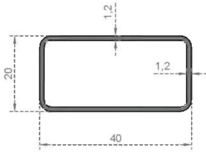
System Code 468 Weight (kg/mt) 0,362
