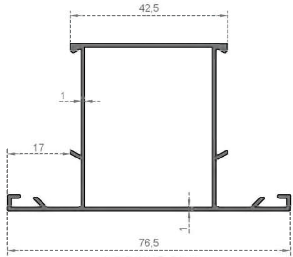
MEETING RAIL
