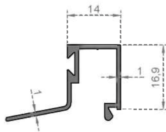
THERMAL INSULATING GLASS BEAM
