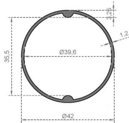
System Code 817 Weight (kg/mt) 0,457
