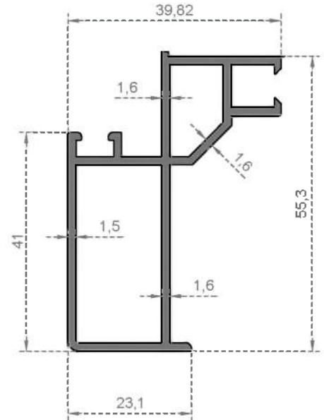
System Code 506 Weight (kg/mt) 0,835
