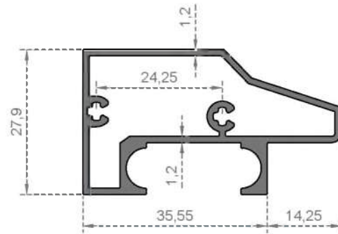
System Code 2948 Weight (kg/mt) 0,651
