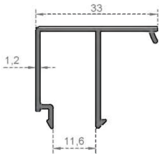
System Code 4020 Weight (kg/mt) 0,308
