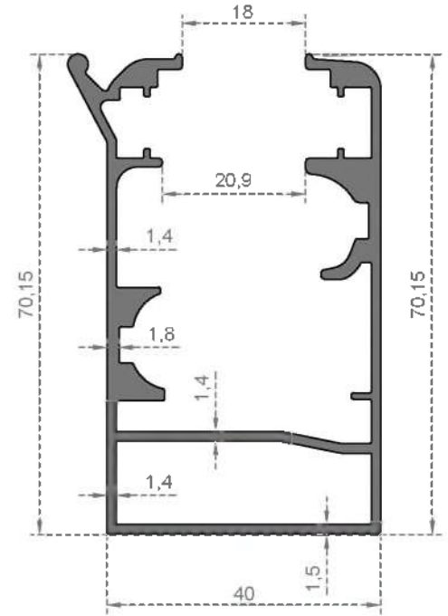
System Code 244 Weight (kg/mt) 1,351
