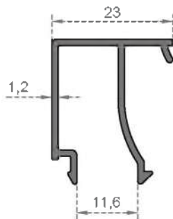
System Code 4025 Weight (kg/mt) 0,279
