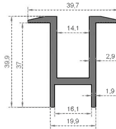
System Code 6726 Weight (kg/mt) 0,805
