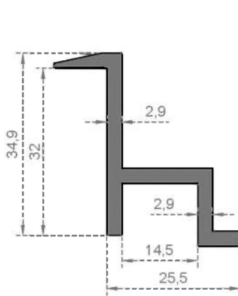
System Code 6725 Weight (kg/mt) 0,605
