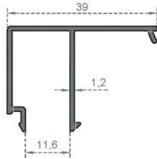
System Code 4017 Weight (kg/mt) 0,330
