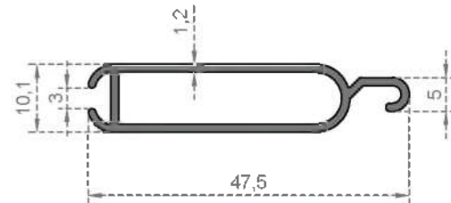
System Code 5029 Weight (kg/mt) 0,339
