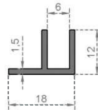
System Code 3104 Weight (kg/mt) 0,160
