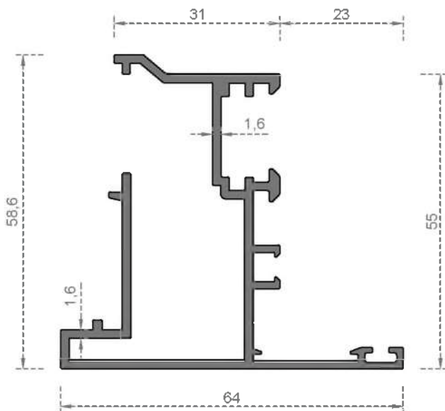
System Code 8008 Weight (kg/mt) 1,035
