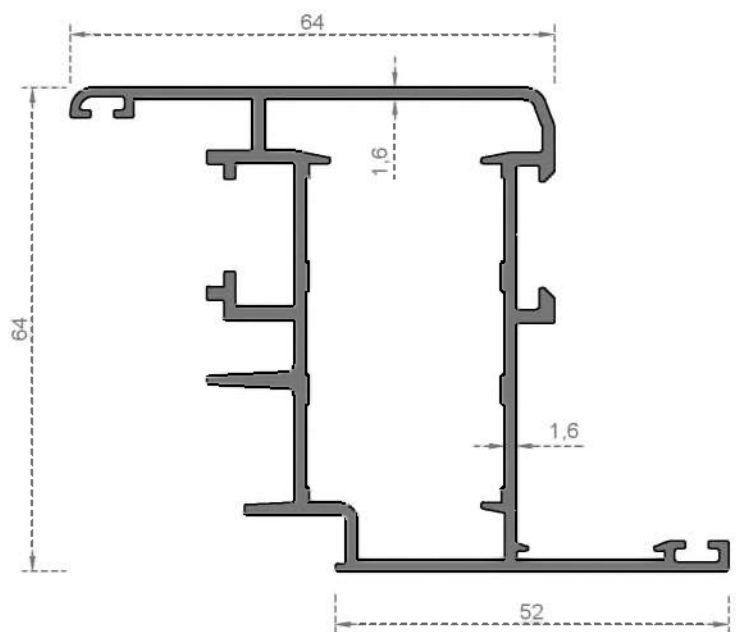
System Code 8003 Weight (kg/mt) 1,417
