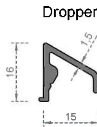
System Code 8010 Weight (kg/mt) 0,171
