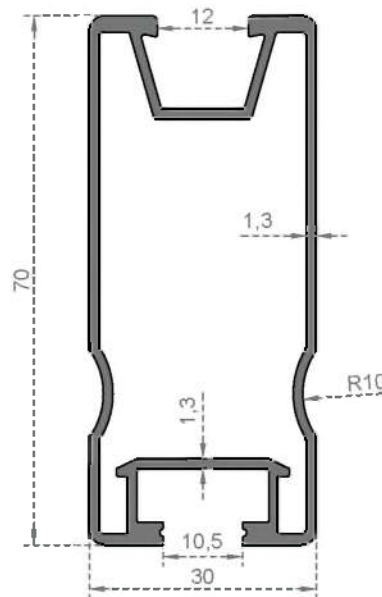
System Code 6728 Weight (kg/mt) 0,940
