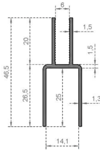
System Code 2995 Weight (kg/mt) 0,395
