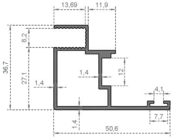
System Code 234 Weight (kg/mt) 0,615
