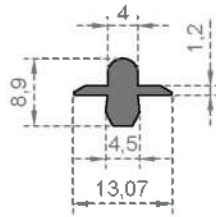
System Code 6058 Weight (kg/mt) 0,118
