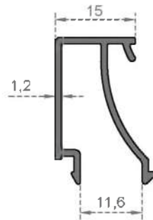
System Code 4029 Weight (kg/mt) 0,257
