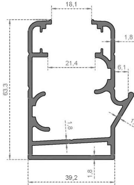
System Code 216 Weight (kg/mt) 1,372
