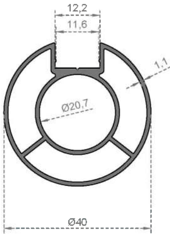
System Code 7046 Weight (kg/mt) 0,660
