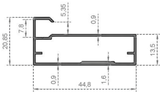
System Code 831 Weight (kg/mt) 0,358
