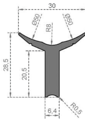
System Code 7053 Weight (kg/mt) 0,545
