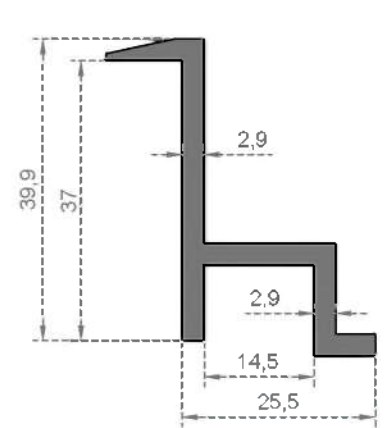
System Code 6727 Weight (kg/mt) 0,645
