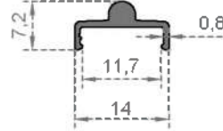
System Code 6380 Weight (kg/mt) 0,077
