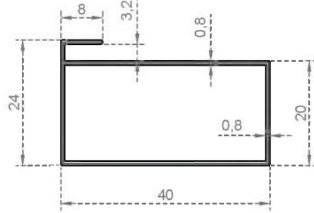
System Code 803 Weight (kg/mt) 0,278
