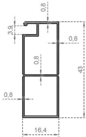
System Code 5563 Weight (kg/mt) 0,298
