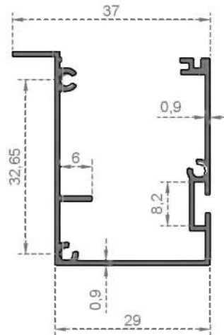
System Code 6532 Weight (kg/mt) 0,387
