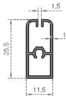
System Code 2992 Weight (kg/mt) 0,236
