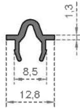
System Code 5698 Weight (kg/mt) 0,103
