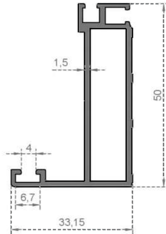
System Code 505 Weight (kg/mt) 0,631
