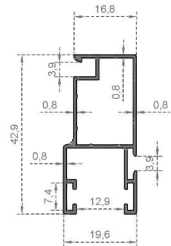
System Code 5869 Weight (kg/mt) 0,340
