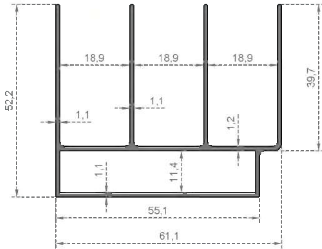
System Code 254 Weight (kg/mt) 0,900
