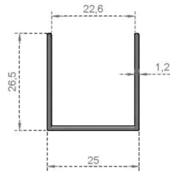
System Code 2988 Weight (kg/mt) 0,245
