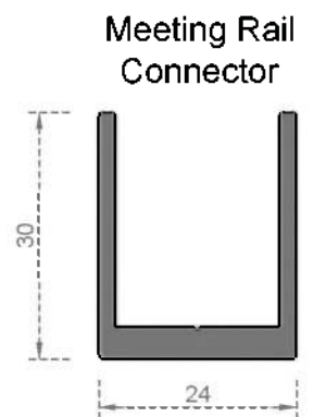
System Code 8011 Weight (kg/mt) 0,545
