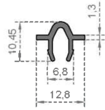
System Code 6705 Weight (kg/mt) 0,100
