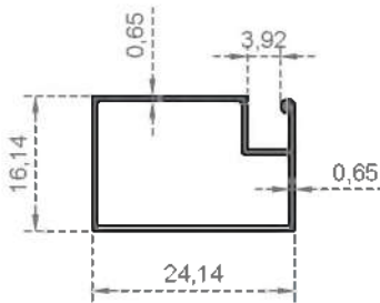
System Code 5272 Weight (kg/mt) 0,154
