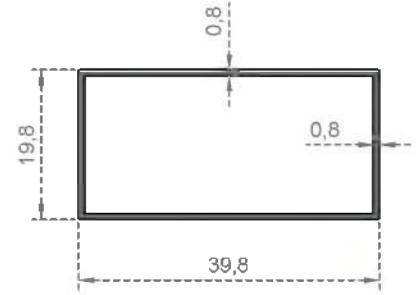
System Code 5304 Weight (kg/mt) 0,252
