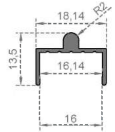
System Code 6947 Weight (kg/mt) 0,135
