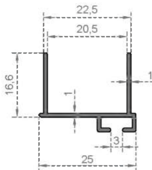
System Code 1733 Weight (kg/mt) 0,185
