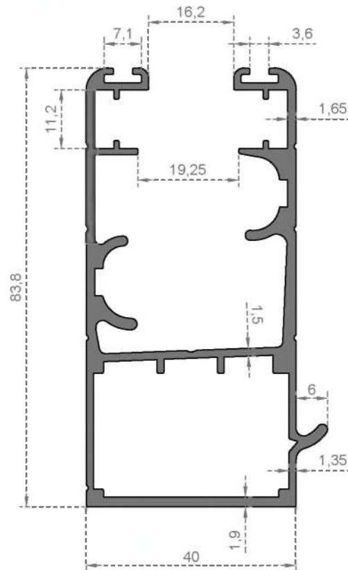
System Code 229 Weight (kg/mt) 1,592
