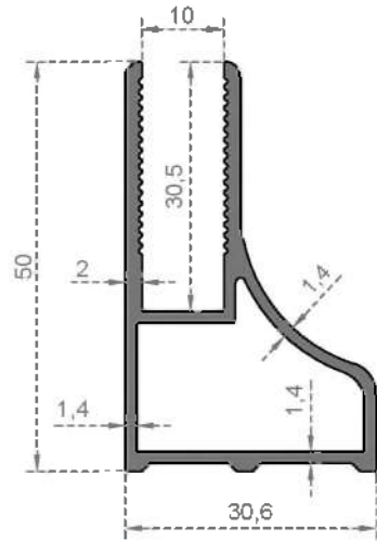
System Code 7035 Weight (kg/mt) 0,825
