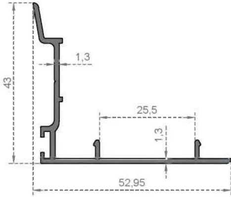
System Code 415 Weight (kg/mt) 0,400
