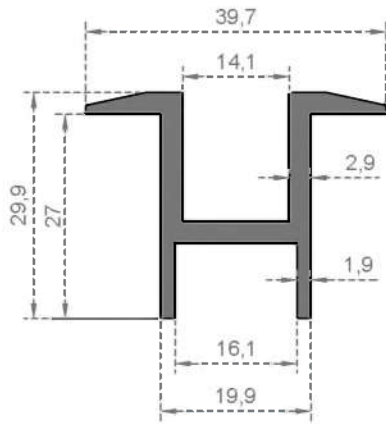
System Code 6722 Weight (kg/mt) 0,645
