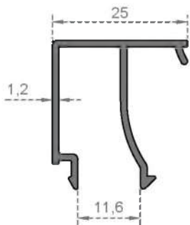
System Code 4024 Weight (kg/mt) 0,286
