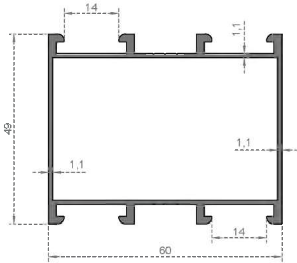
FRAME
