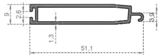
System Code 5027 Weight (kg/mt) 0,397
