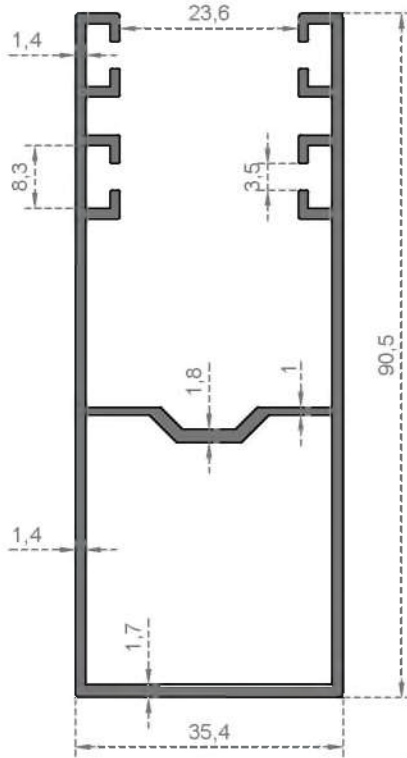
System Code 5026 Weight (kg/mt) 1,172
