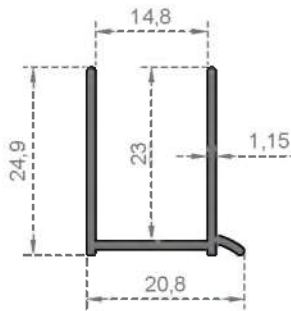
System Code 2985 Weight (kg/mt) 0,215
