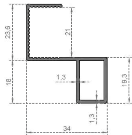
System Code 241 Weight (kg/mt) 0,394
