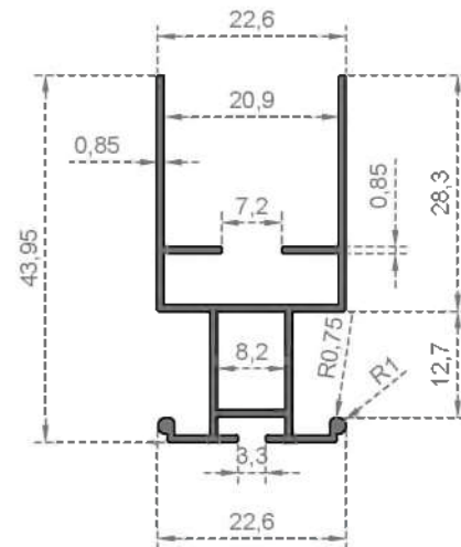
System Code 5034 Weight (kg/mt) 0,355
