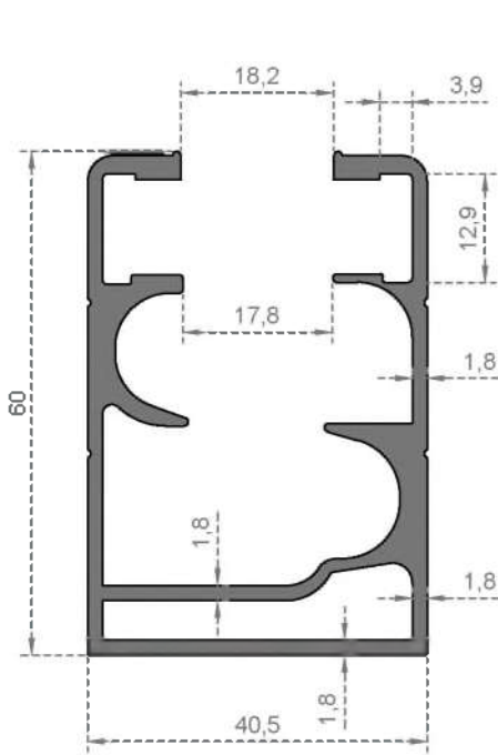
System Code 220 Weight (kg/mt) 1,425
