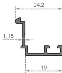
System Code 3003 Weight (kg/mt) 0,172
