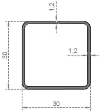
System Code 467 Weight (kg/mt) 0,362
