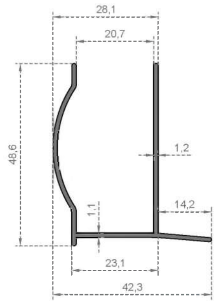
System Code 2226 Weight (kg/mt) 0,419
