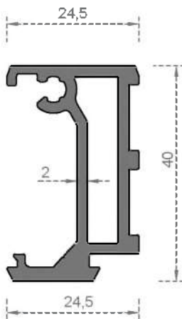
System Code 4014 Weight (kg/mt) 0,775
