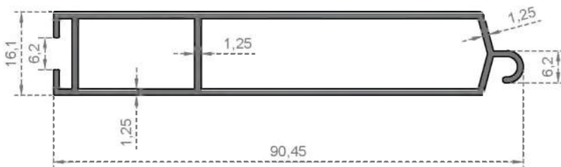
System Code 5024 Weight (kg/mt) 0,760
