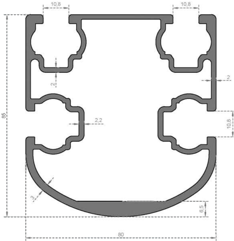
System Code 6744 Weight (kg/mt) 3,280
