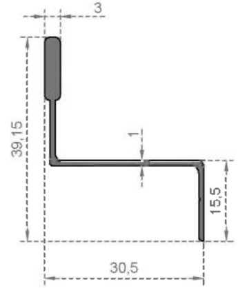
System Code 5567 Weight (kg/mt) 0,248
