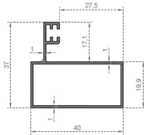
System Code 233 Weight (kg/mt) 0,420
