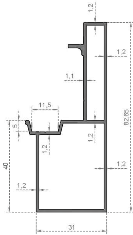
System Code 2994 Weight (kg/mt) 0,815
