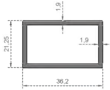
System Code 230 Weight (kg/mt) 0,555
