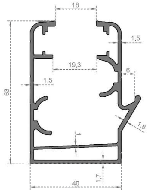
System Code 238 Weight (kg/mt) 1,199
