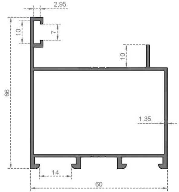
CASEMENT
