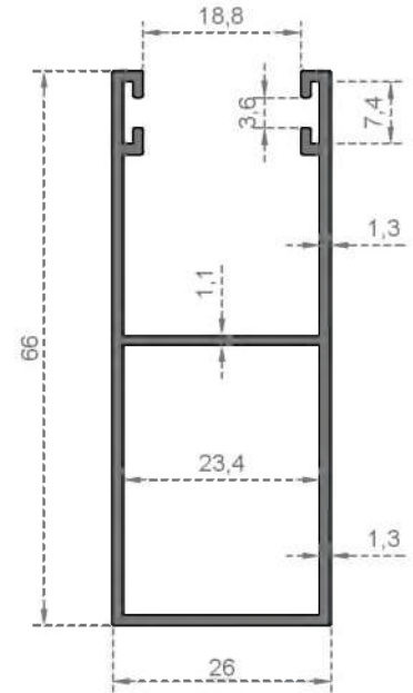
System Code 5036 Weight (kg/mt) 0,675
