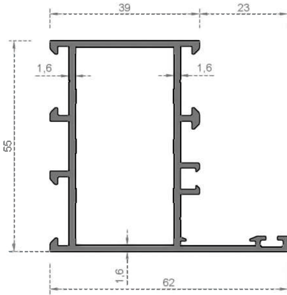
System Code 8000 Weight (kg/mt) 1,078
