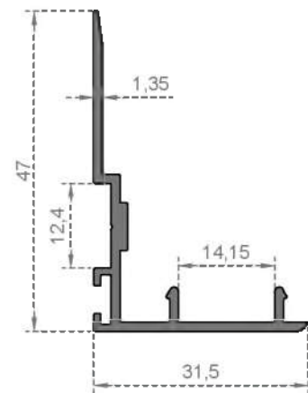
System Code 3004 Weight (kg/mt) 0,356
