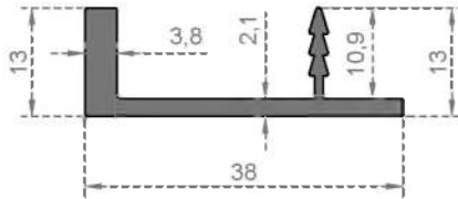
System Code 808 Weight (kg/mt) 0,372
