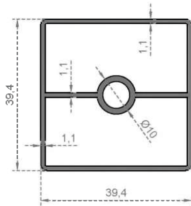
System Code 818 Weight (kg/mt) 0,642
