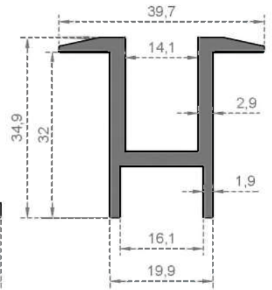
System Code 6724 Weight (kg/mt) 0,725
