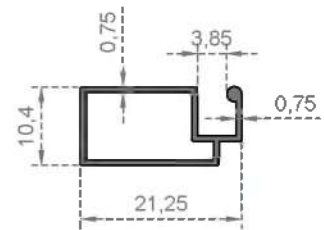
System Code 5868 Weight (kg/mt) 0,135
