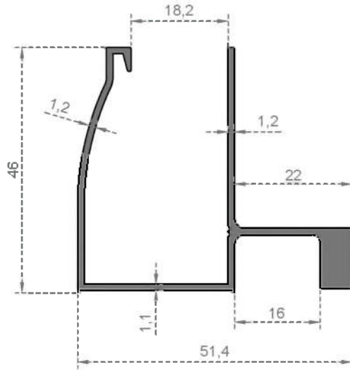
System Code 2905 Weight (kg/mt) 0,640
