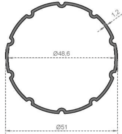
System Code 816 Weight (kg/mt) 0,551
