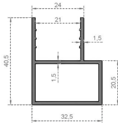
System Code 6686 Weight (kg/mt) 0,580
