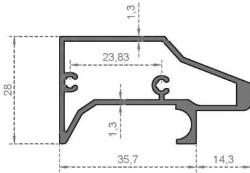
System Code 2903 Weight (kg/mt) 0,656
