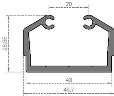
System Code 513 Weight (kg/mt) 0,865
