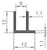
System Code 2997 Weight (kg/mt) 0,095
