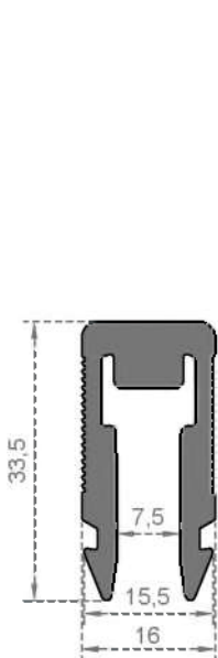
System Code 6733 Weight (kg/mt) 0,742
