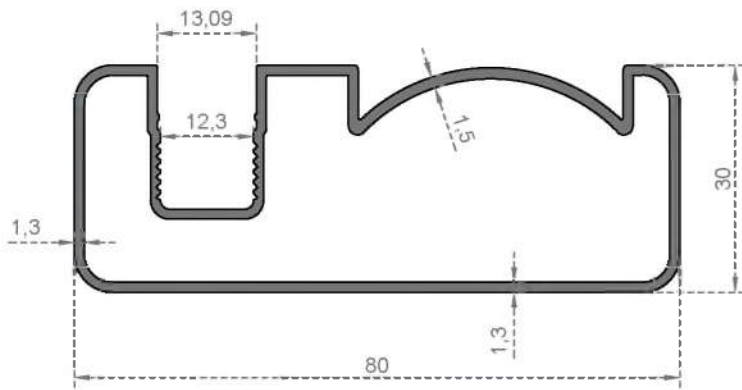
System Code 7039 Weight (kg/mt) 0,940
