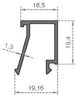
System Code 3002 Weight (kg/mt) 0,246
