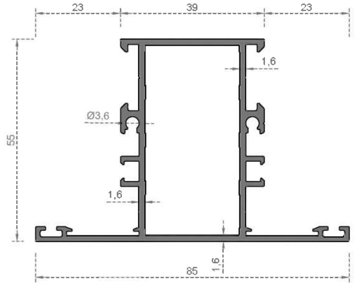
System Code 8001 Weight (kg/mt) 1,243
