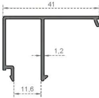
System Code 4016 Weight (kg/mt) 0,335
