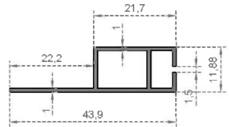
System Code 2990 Weight (kg/mt) 0,254
